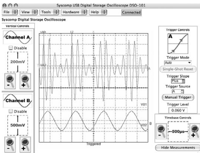
Figure 3 Oscilloscope displaying amplitude modulation
