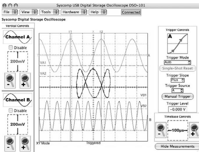
Figure 2 Oscilloscope with two sine wave inputs plus XY plot
