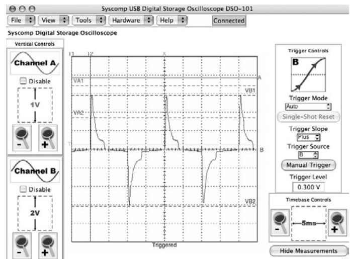
Figure 4 Oscilloscope displaying compact fluorescent lamp current waveform
