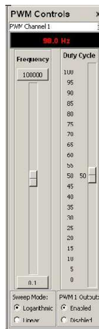
Figure 6: Pulse Generator Control Panel
