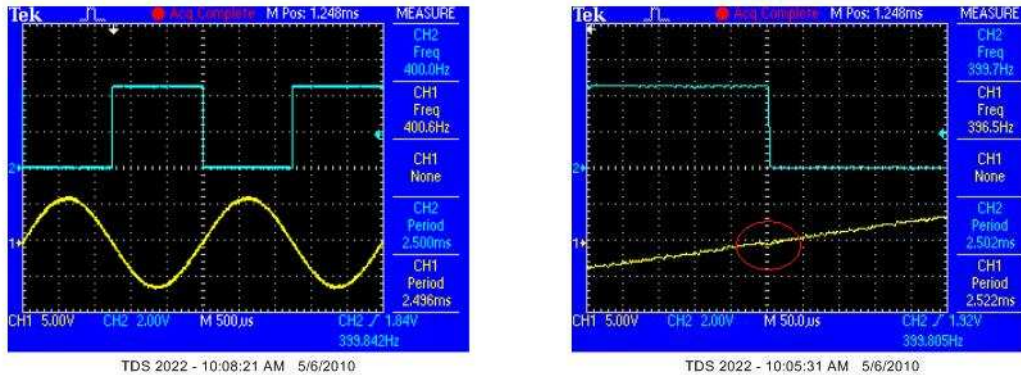
(a) Waveforms
